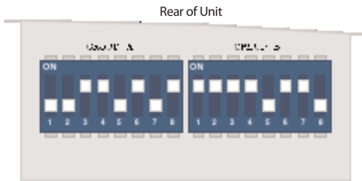
Inside Switch Compartment (default settings)
